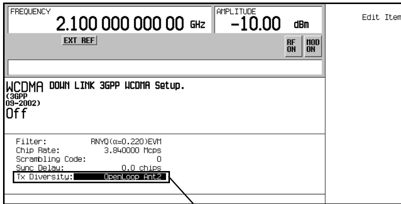
Figure 14-18 Antenna Two Selection
