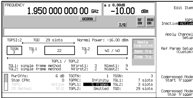
Figure 15-61 TGPSI 2 Setup
