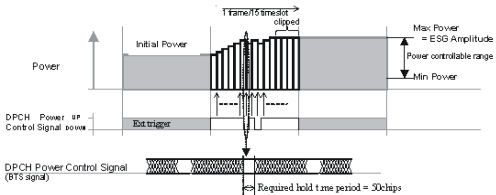
Figure 15-89 DPCH External Power Control
