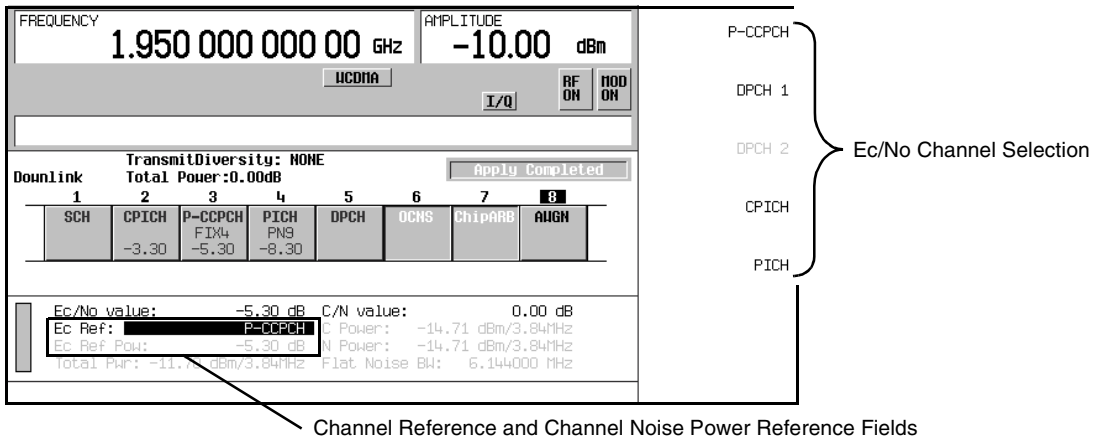
Figure 14-36 E_c/N_o Reference Selection
