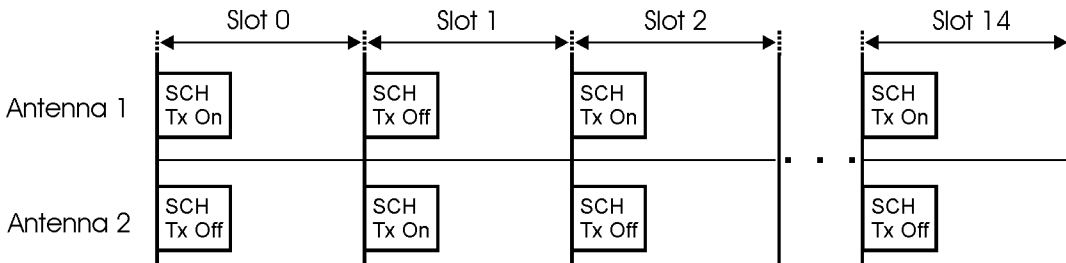
Figure 14-9 SCH TSTD Operation
