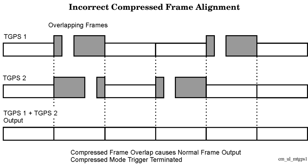
Figure 15-54 Multiple TGPS Compressed Frame Alignment
