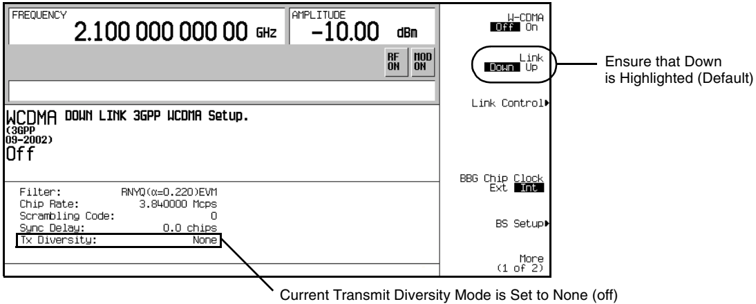
Figure 14-20 First-Level W-CDMA Softkey Menu
