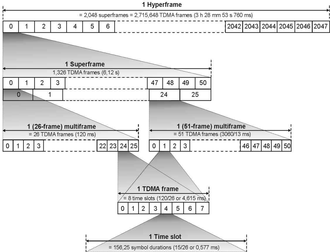
Figure 12-2 Multiframe Hierarchy
