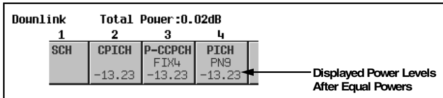
Figure 14-5 Equal Powers
