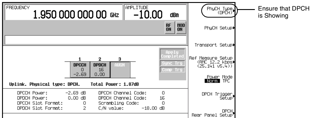
Figure 15-49 DPCH is Selected
