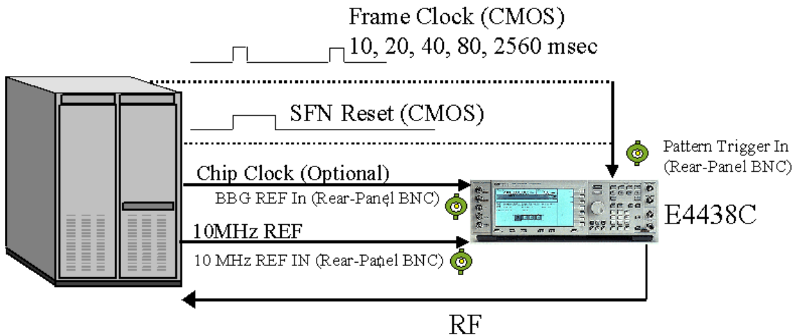
Figure 15-73 Cable Connections
