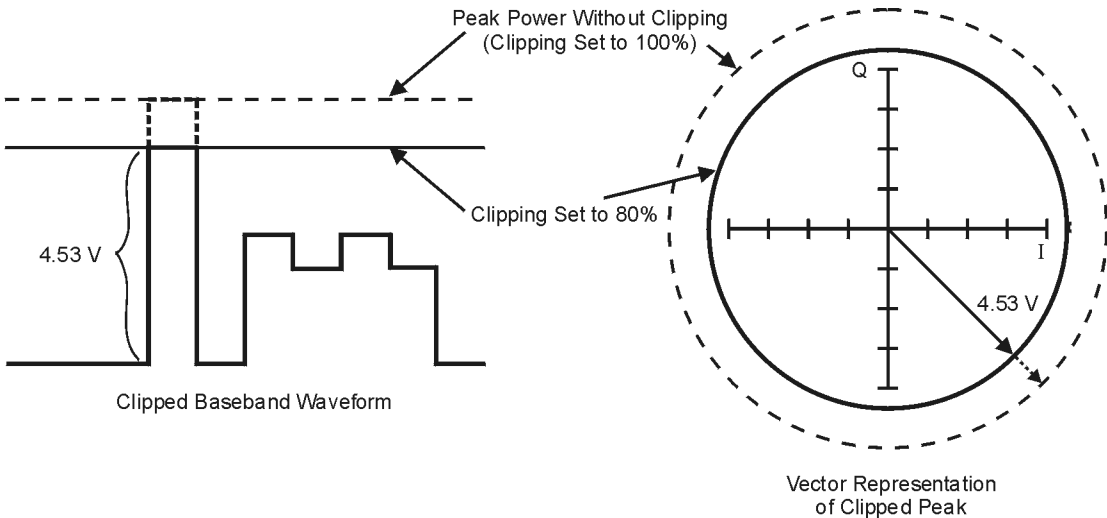
Figure 3-19 Circular Clipping
