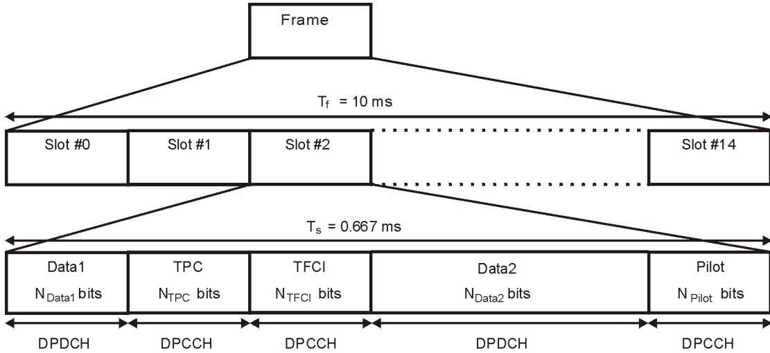
Figure 14-39 DPCCH/DPDCH Frame Structure
