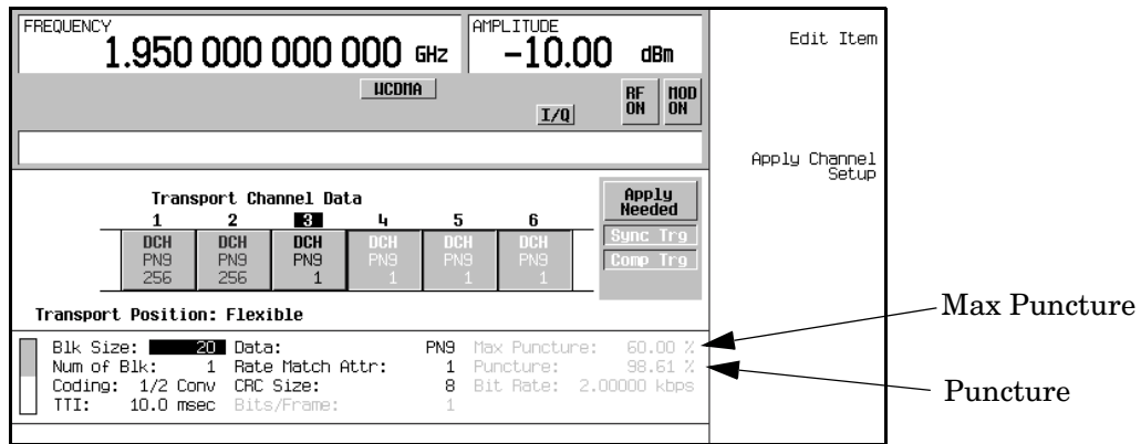
Figure 15-41 Excessive Puncturing
