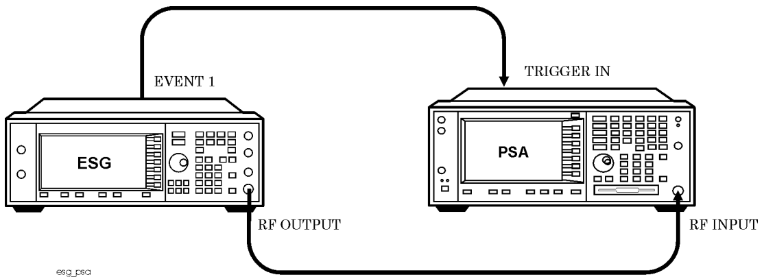
Figure 15-1 PSA Setup
