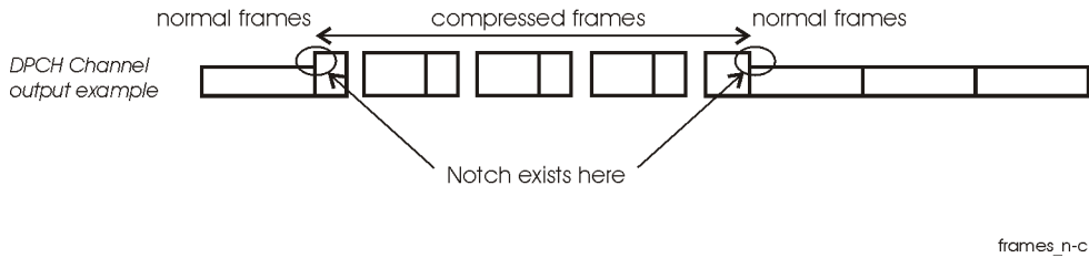
Figure 15-71 RF Notch with Compressed Mode Transitions
