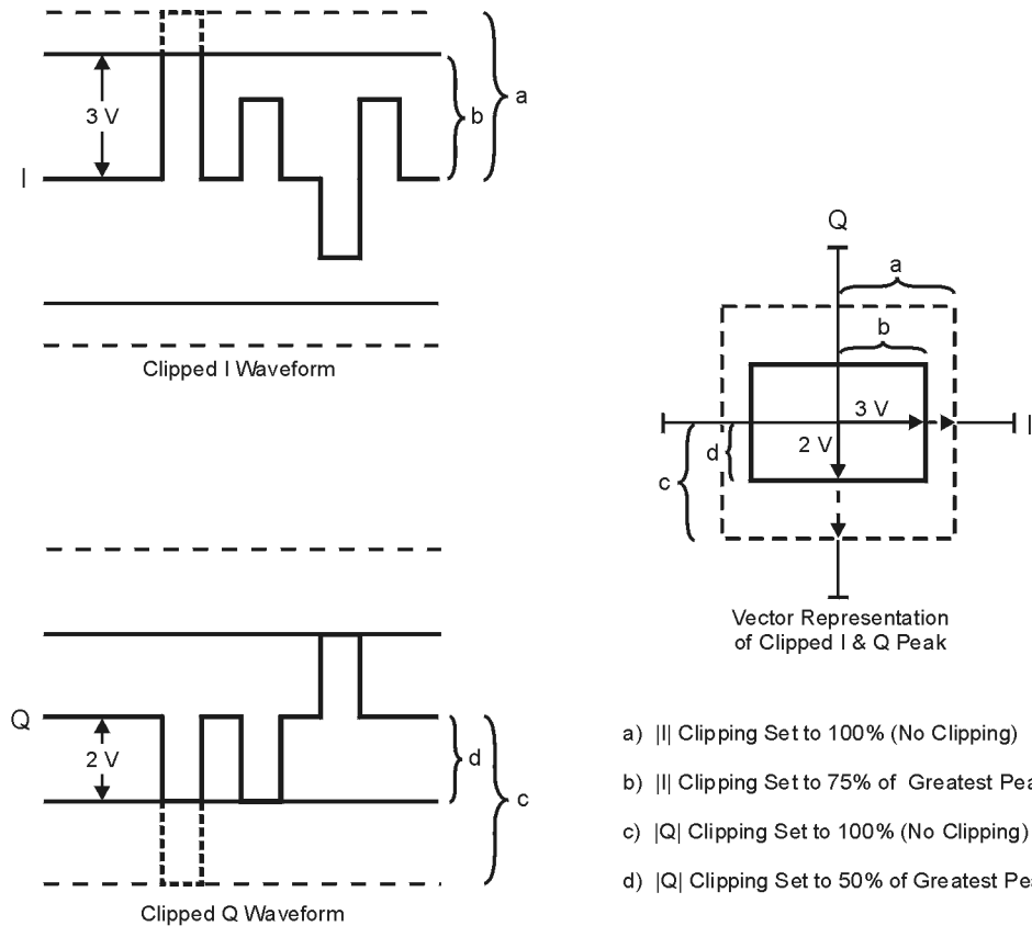
Figure 3-20 Rectangular Clipping
