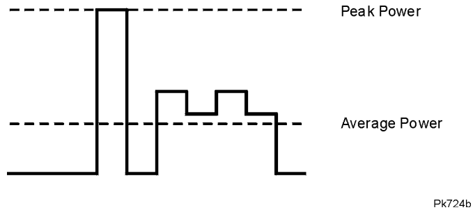
Figure 3-17 Peak-to-Average Power in the CDMA Waveform
