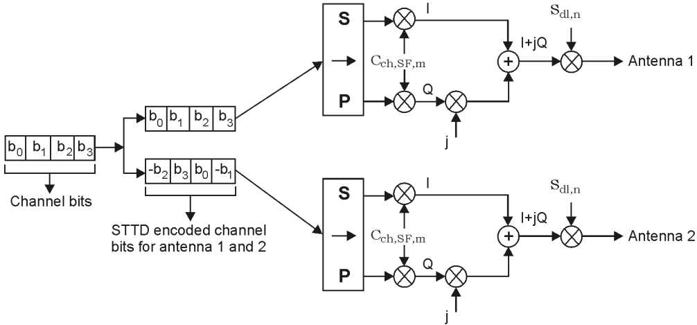
Figure 14-8 Generic STTD Encoder
