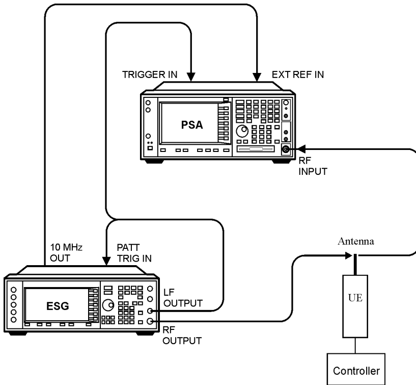
Figure 14-19 Out-of-Synchronization Setup
