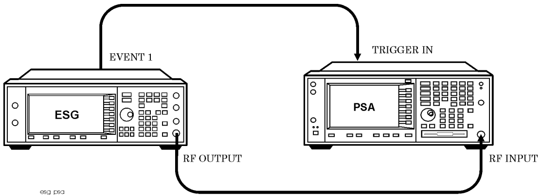
Figure 15-47 PSA Setup
