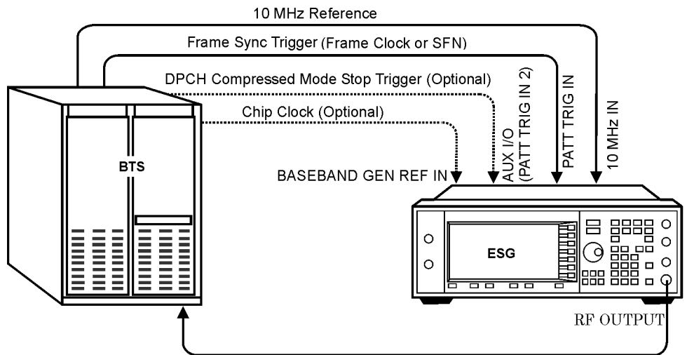
Figure 15-2 Base Transceiver Station Setup
