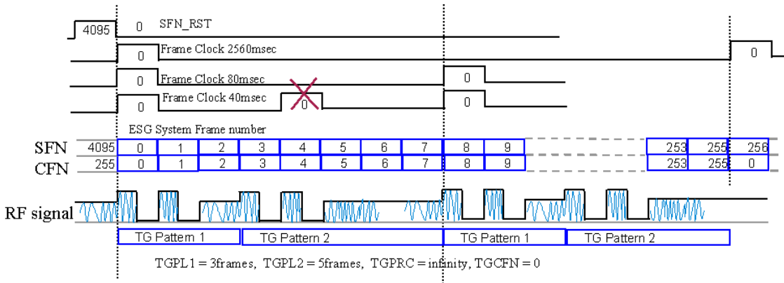
Figure 15-81 DPCCH Synchronization - Frame Number Alignment for Continuous (Infinity) Compressed Mode
