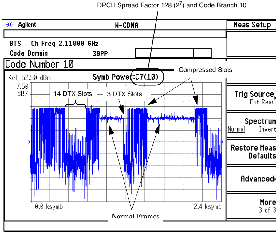
Figure 14-30 Compressed DPCH Signal
