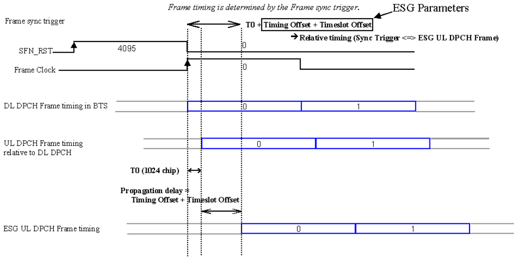
Figure 15-79 DPCH Synchronization - Frame Timing Alignment
