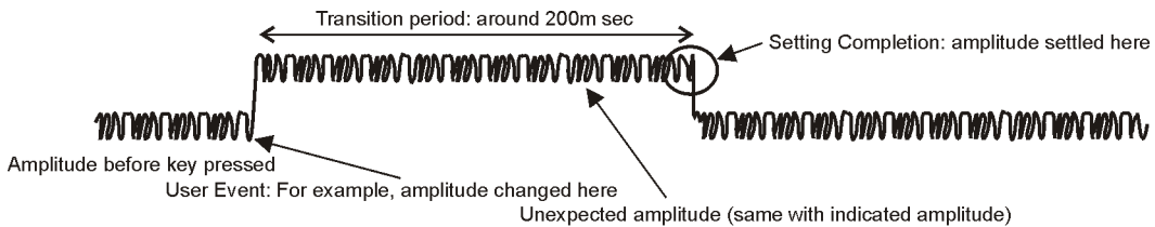
Figure 15-72 DPCH Compressed Mode Signal after a Change in Amplitude
