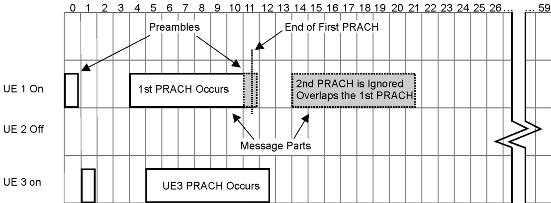
Figure 15-21 Transmitting PRACHs
