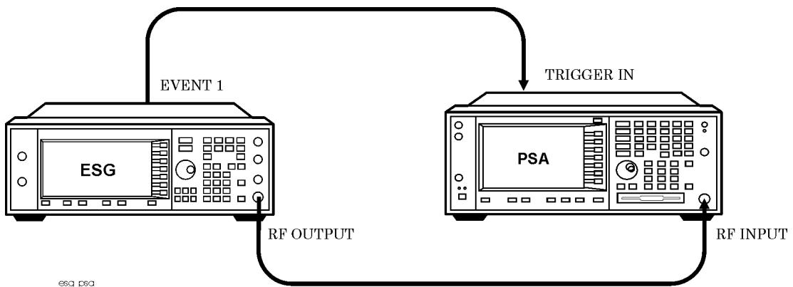
Figure 15-55 PSA Setup
