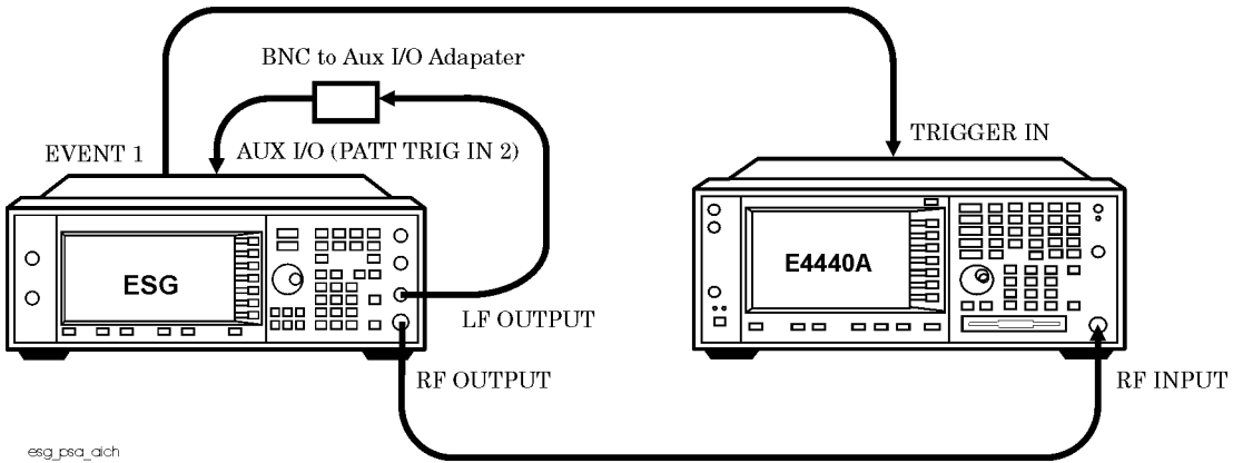
Figure 15-17 AICH Connection Diagram
