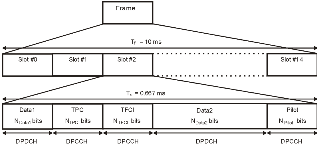
Figure 13-11 DPCCH/DPDCH Frame Structure
